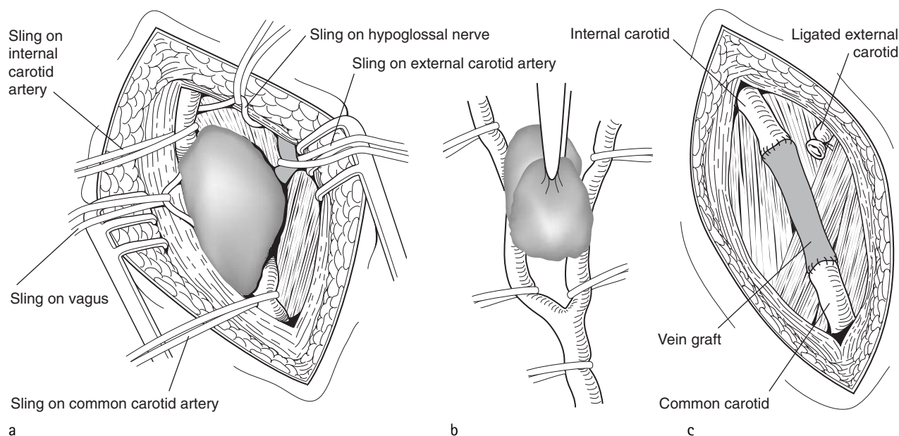
Figure 6.25 Carotid body tumour. (a) Tapes have been placed around the common, internal and external carotid arteries, and around the vagus and hypoglossal nerves. (b) The tumour is dissected off the vessels in the sub-adventitial plane. (c) When the arteries have to be excised with the tumour, the external carotid is ligated but a graft is interposed between the common and internal carotid arteries.
